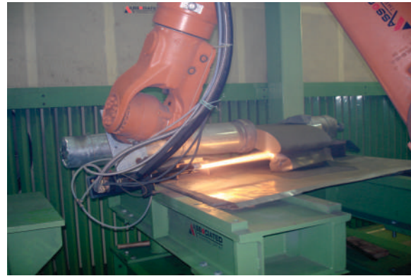
Robotic Coating on Guide Vane
